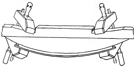
FIG. 403. BENDING CHAIR-BACK SLAT.
